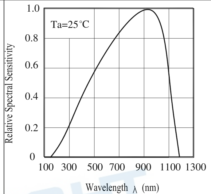
Spectral Sensitivity
