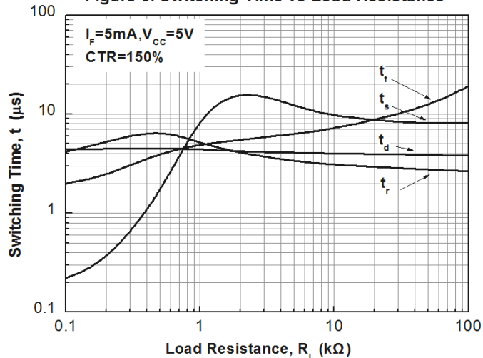
Figure 6. Switching Time vs Load Resistance
