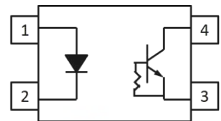
Pin Configuration
