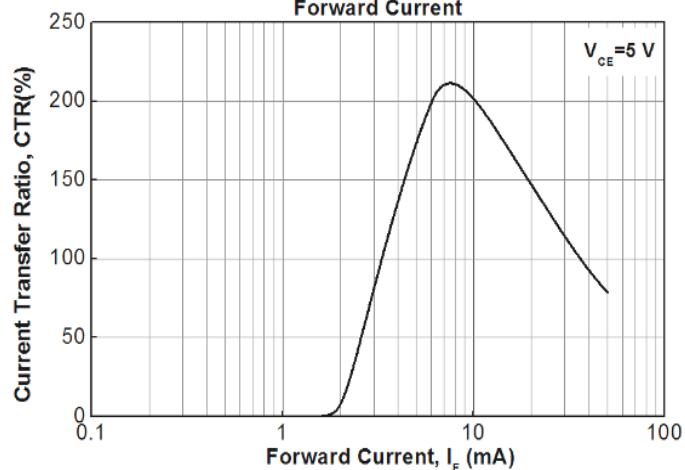
Figure 2. Current Transfer Ratio vs Forward Current
