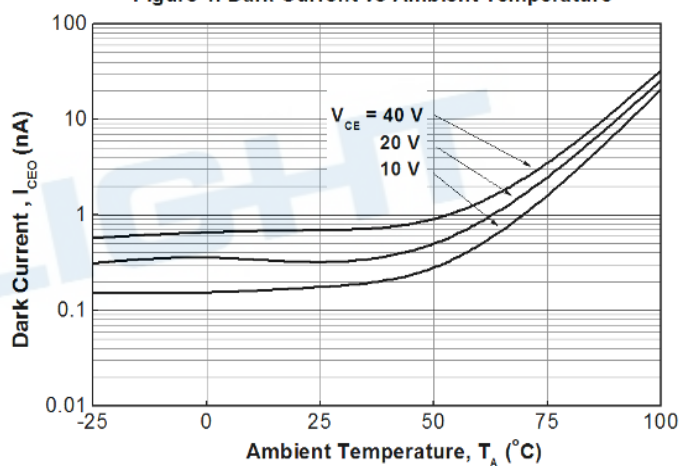
Figure 4. Dark Current vs Ambient Temperature
