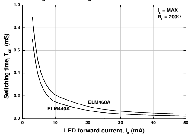
Figure 4. Switching time vs LED forward current
