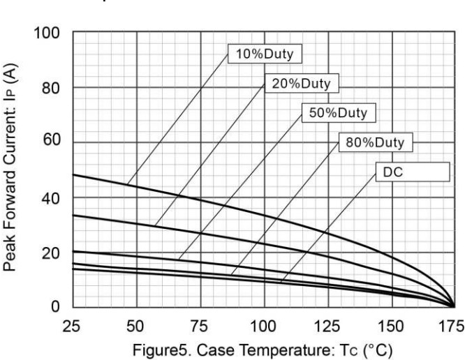
Maximum I P -T C Characteristics
