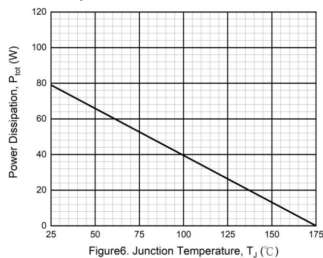
Power Dissipation
