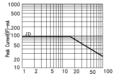
Fig6. MAX. PEAK CURRENT VS. DUTY CYCLE % (REFRESH RATE 1KHz)
