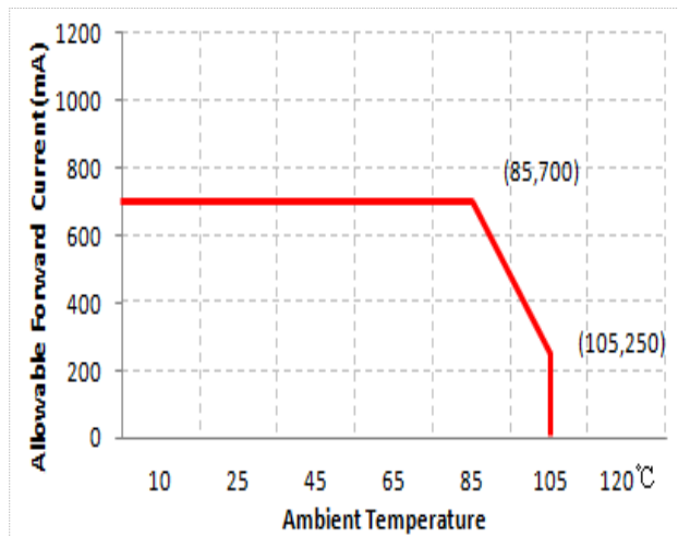
Fig 8. Ambient Temperature vs.Maximum Forward Current - Red
