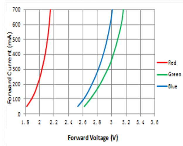
Fig 4. Forward Current vs. Forward Voltage, T_a = 25^\circ\text{C}
