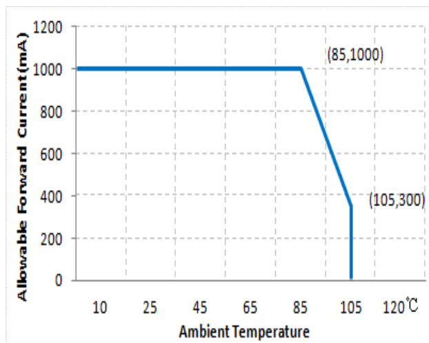
Fig 10. Ambient Temperature vs.Maximum Forward Current - Blue
