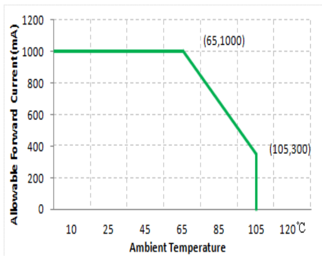
Fig 9. Ambient Temperature vs.Maximum Forward Current - Green
