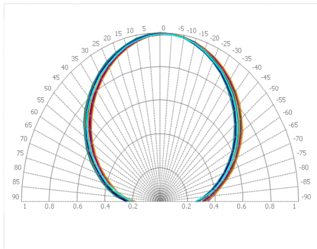
Fig 7. Typical Viewing Angle =120° , Ta = 25℃
