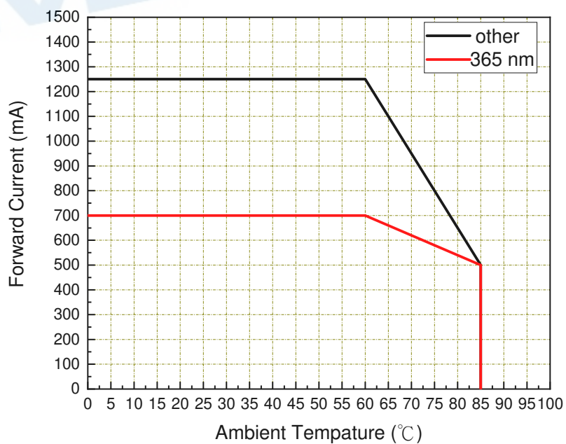
Derating Curve
