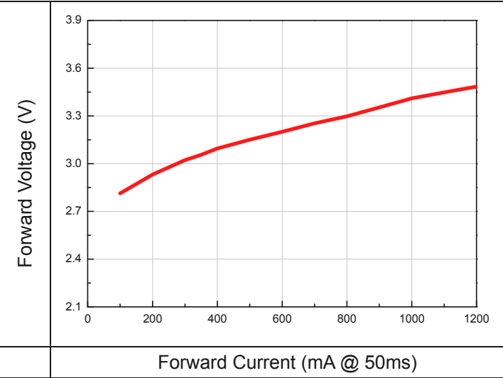
Forward Voltage vs. Forward Current (T solder pad =25°C)
