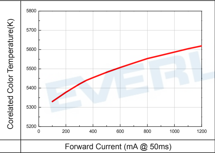
CCT vs. Forward Current (T soldering pad =25°C)
