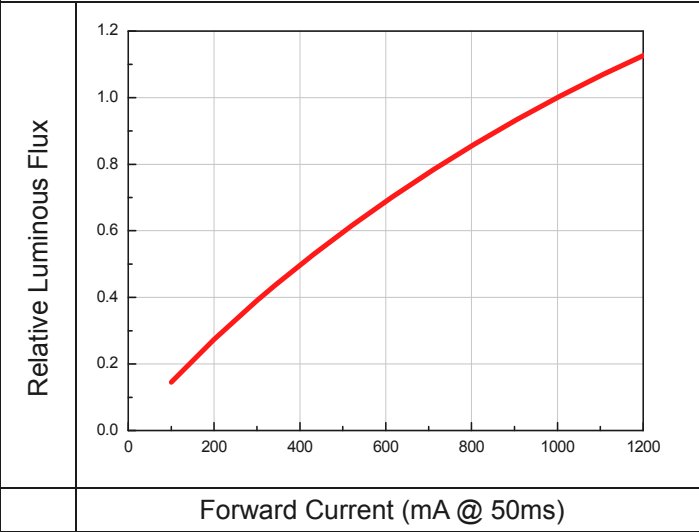
Relative Luminous Flux vs. Forward Current (T solder pad =25°C)
