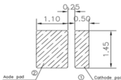
Recommended soldering pattern layout
