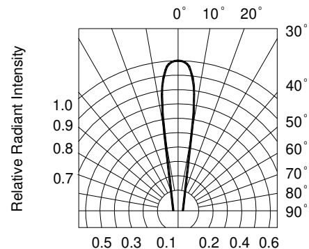
FIG.6 RADIATION DIAGRAM
