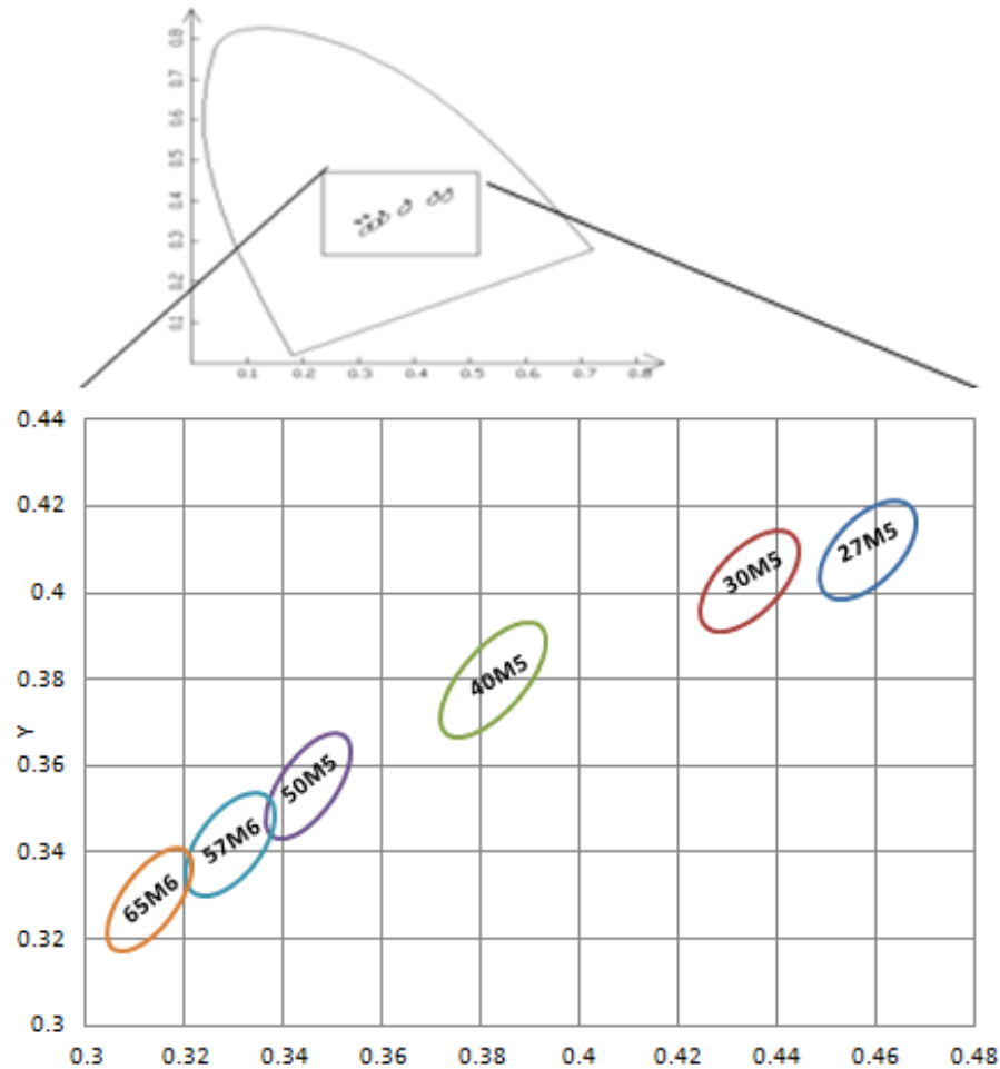
Fig 9, CIE Chromaticity Diagram (CIE色区图), IF = 80mA, Ta = 25℃
