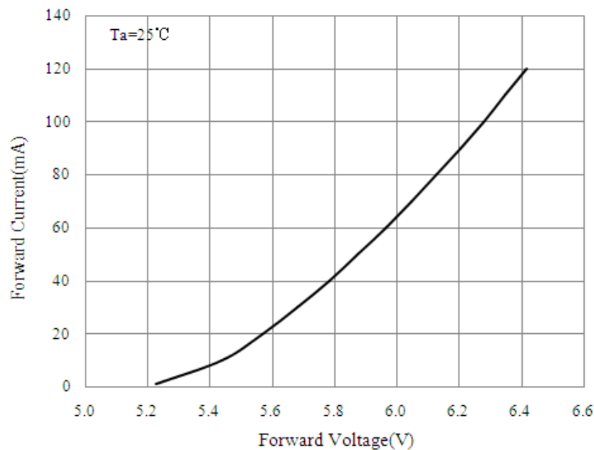
Fig 4. Forward Voltage vs. Forward Current , Ta = 25℃ (电压与电流关系, 温度=25℃)
