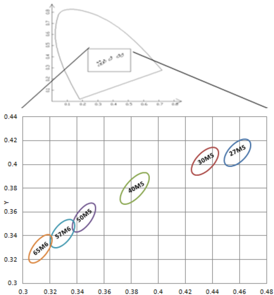
Fig 9, CIE Chromaticity Diagram (CIE色区图), IF = 25mA, Ta = 25℃
