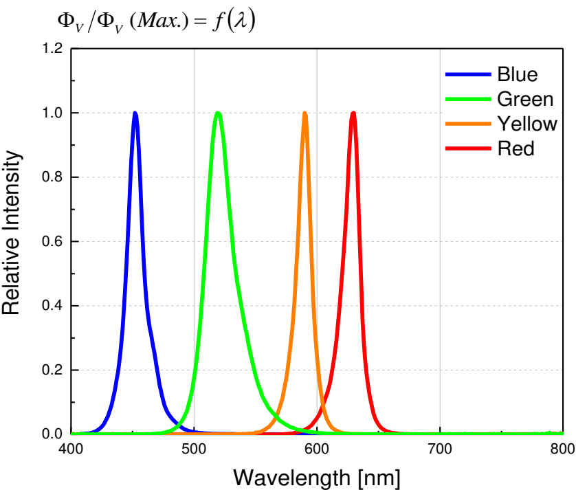
Wavelength Characteristics Relative Spectral Distribution @ Ts = 25°C , If=40mA
