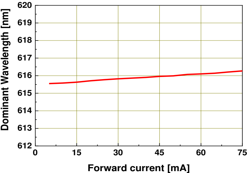
Dominant Wavelength vs. Forward Current @ Ts = 25°C
