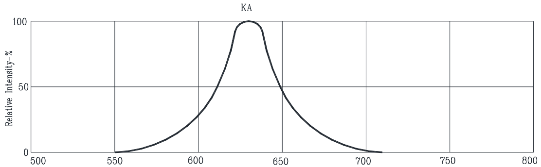
PEAK WAVELENGTH \lambda_p (nm) Fig1. Spectral Emission
