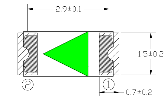
Recommend Sodering Pad
