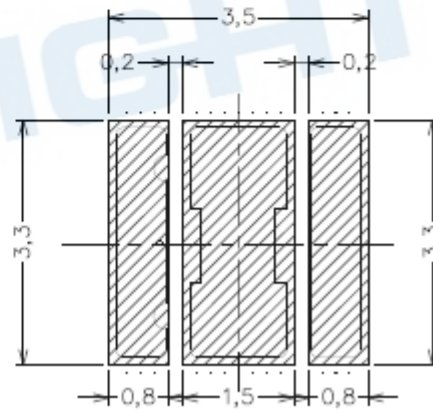
Soldering patterns
