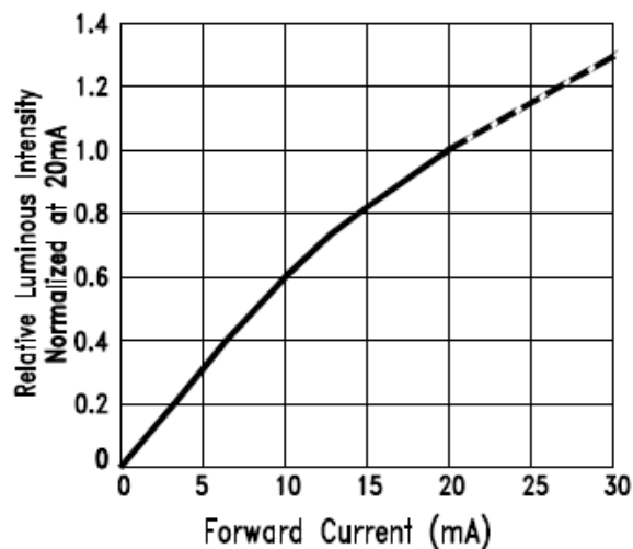
Fig.4 Relative Luminous Intensity
