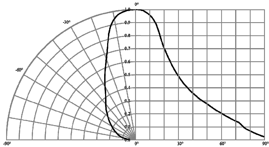
Fig 3. Radiation Characteristics
