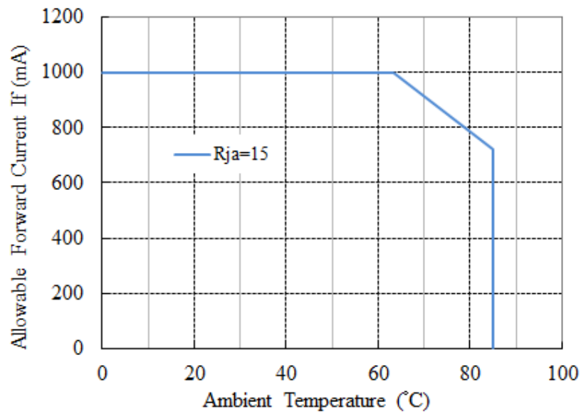
Fig 6. Forward Current Derating Curve
