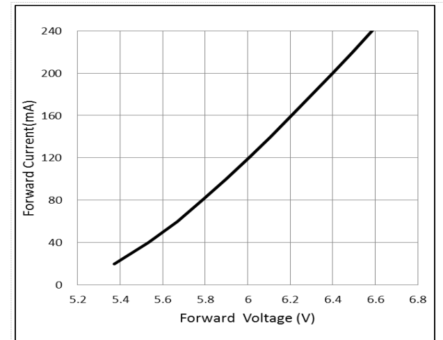
Fig 6. Forward Current vs. Forward Voltage, T_j = 25^\circ\text{C}
